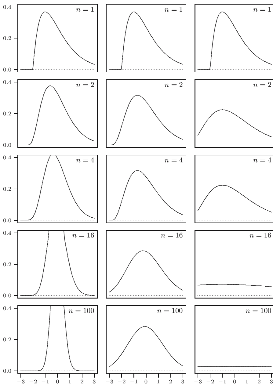
Fig. 14.1. Multiplying the difference \bar{X}_n - \mu of n Gam(2, 1) random variables. Left column: n^{1/4}(\bar{X}_n - \mu) ; middle column: \sqrt{n}(\bar{X}_n - \mu) ; right column: n(\bar{X}_n - \mu) .
